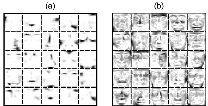
Fig. 1. The learned bases by NMF on (a) CBCL and (b) ORL dataset. A face in (a) CBCL dataset can be successfully decomposed by the learned bases with part-based representation (e.g. nose, eye, mouth, etc.). However, NMF cannot learn these “parts” to represent a face in (b) ORL dataset.
