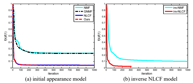
Fig. 9. Objective values versus iteration numbers for NMF variants in (a) the initial appearance model and (b) the inverse NLCF model, where the stopping error is set to 10^{-5} , and the maximal iteration time is fixed to 1000.
