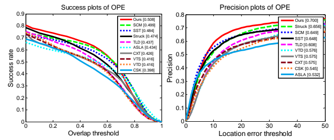
Fig. 5. Plots of OPE. The performance score for each tracker is shown in the legend. For each figure, the top 10 trackers are presented for clarity.
