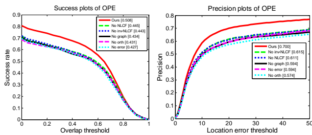
Fig. 8. Plots of OPE. The success plot and precision plot of our proposed tracker versus different regularization terms, where “No graph” is associated with \lambda , “No error” is with respect to \beta , “No NLCF” is with \mu , and “No orth” relates to \gamma in Eq. (6). \zeta is the regularization parameter in inv-NLCF model associated to “No inv-NLCF”.
