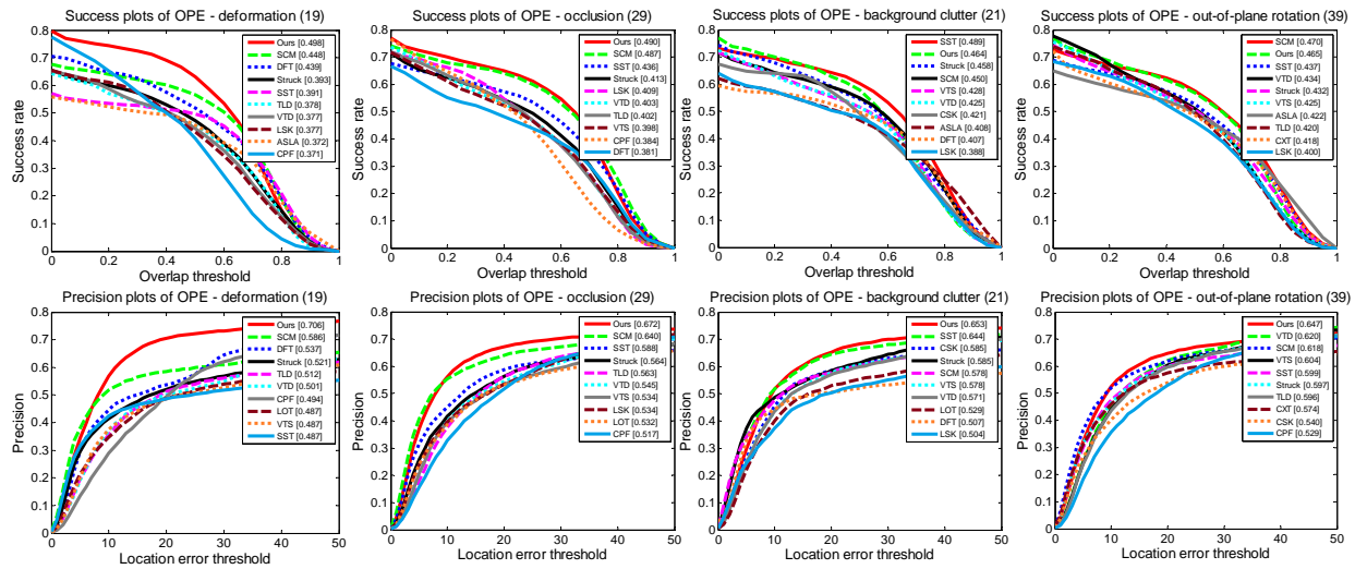
Fig. 6. Success plots and precision plots of OPE on four main attributes ( Deformation, Occlusion, Background Clutter, and Out-of-plane Rotation ).
