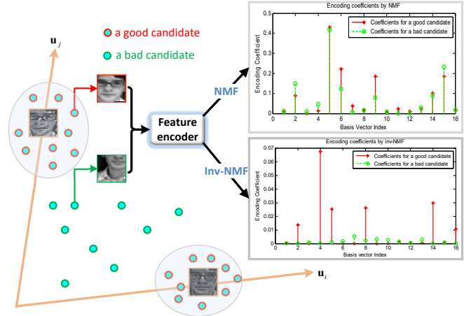
Fig. 4. Encoding coefficients obtained by NMF and inv-NMF feature coder. In NMF coding scheme, the encoding coefficients for a “good” candidate or a “bad” candidate are similar and thus lacking discriminative ability. In our inv-NMF coding scheme, a “good” candidate distributes near a base vector, which indicates that this candidate resembles certain base vectors with high response values. Whilst a “bad” candidate spreads over the whole space, and has extremely low response values to all these base vectors.
