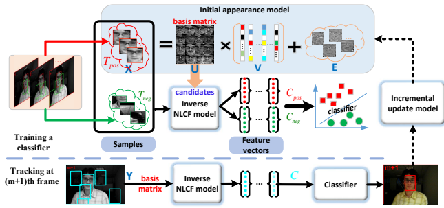
Fig. 3. Flowchart of the proposed tracker.
